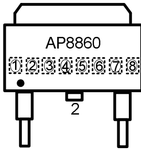
TO-252 (Top View)
