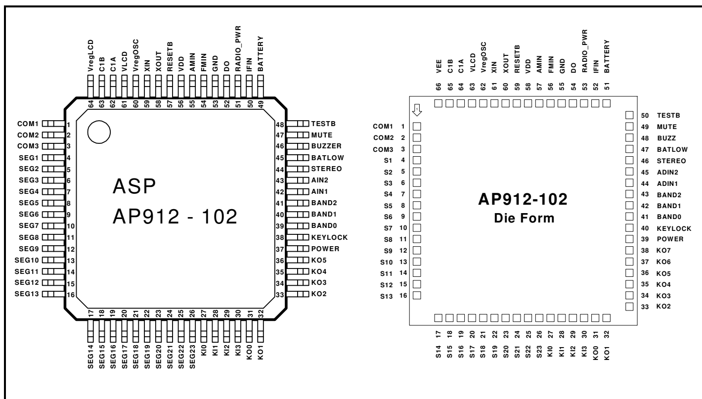
Figure 1. 64 Pin LQFP Package
