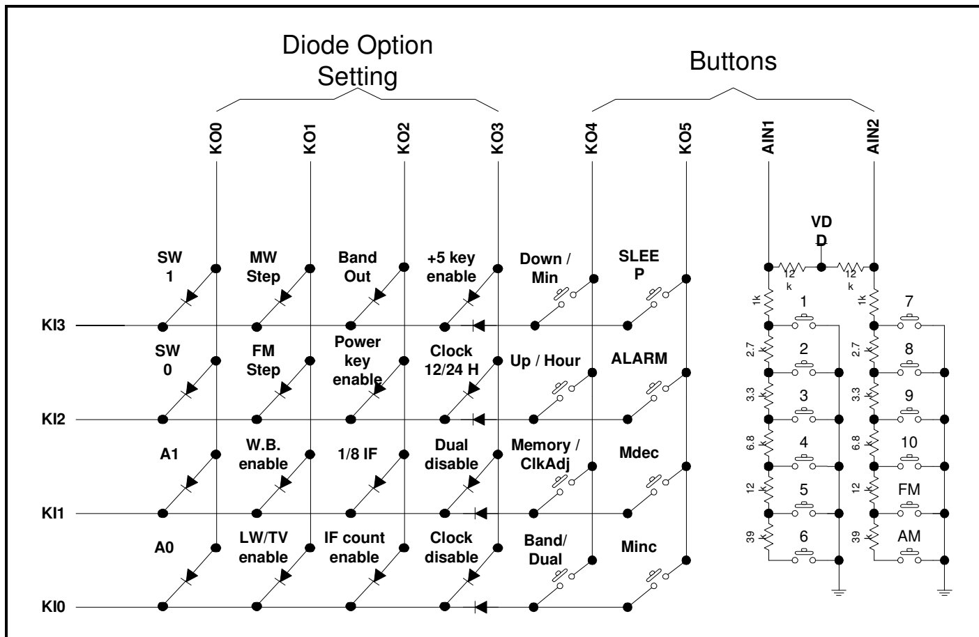
Figure 4. Keyboard Layout
