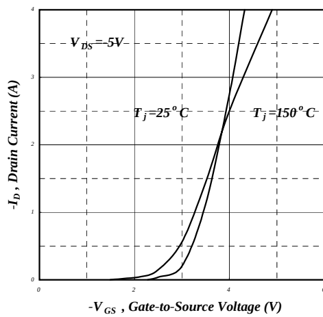
Fig 11. Transfer Characteristics
