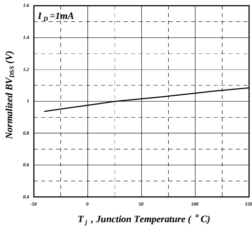
Fig 3. Normalized BV_{DS} vs. Junction Temperature
