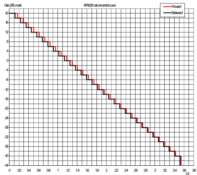
Figure 3: Gain setting vs VOLUME pin voltage
