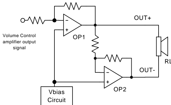
Figure 1: APA2065 internal configuration (each channel)
