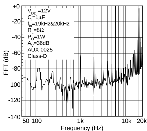
Inter-modulation Performance
