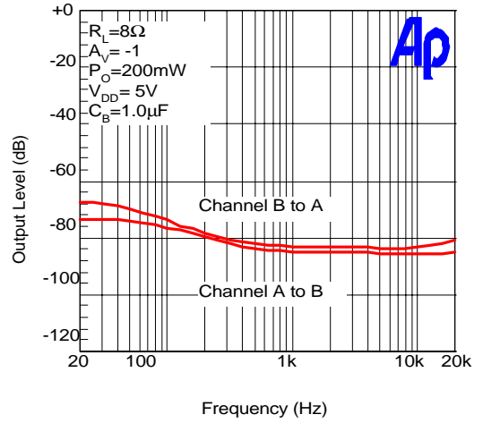
Channel Separation
