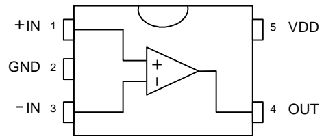
SOT-23-5 (Top View)
