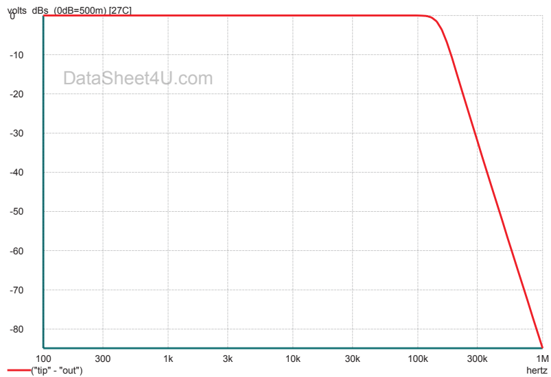
APC77101 FILTER RESPONSE
