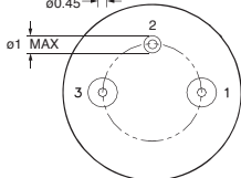
Pin Circle Dia = 7.5
