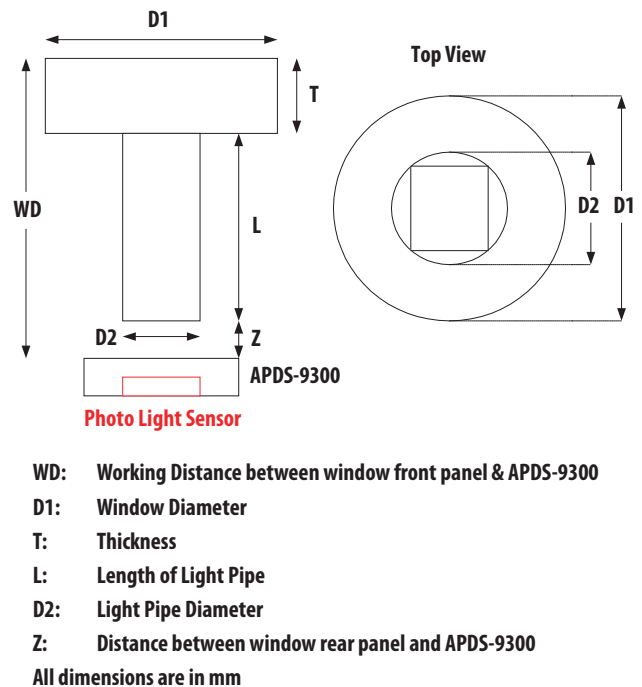
Figure A2. Recommended Window Dimensions
