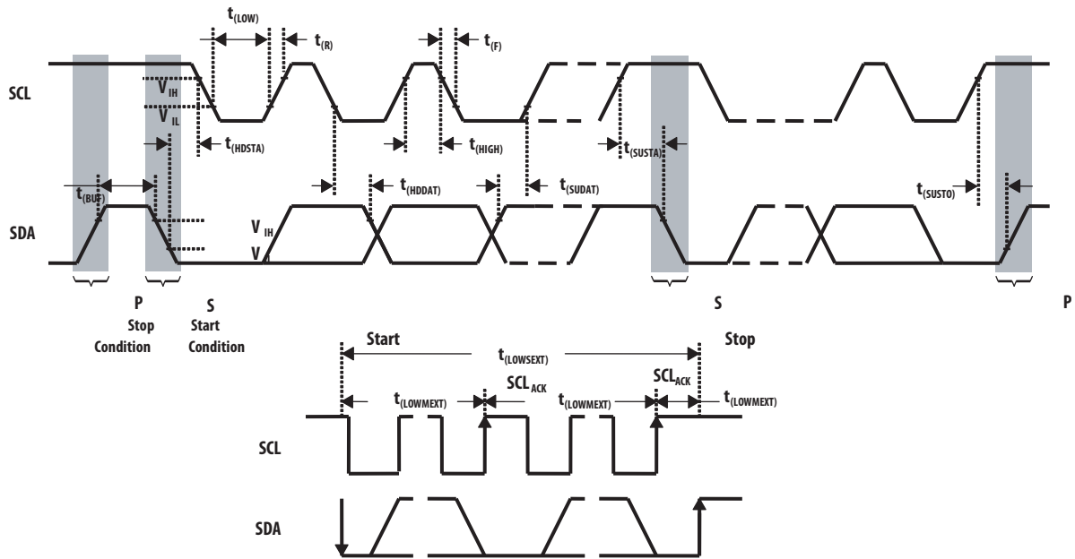
Figure 1. Timing Diagrams
