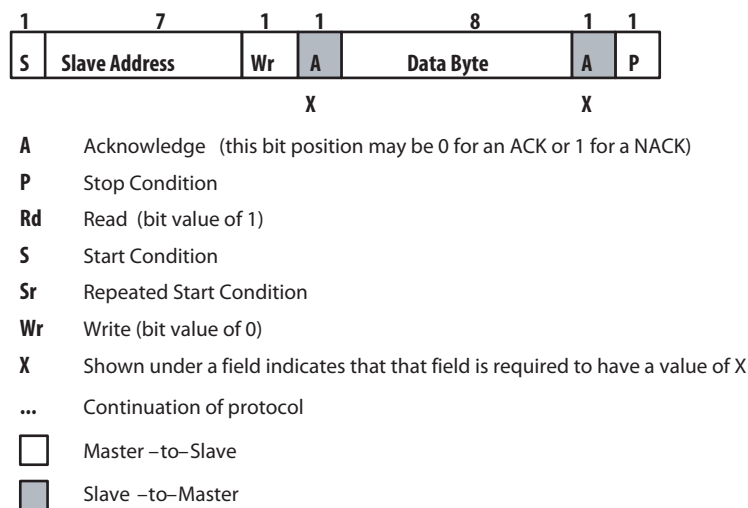
Figure 6. I 2 C Packet Protocol Element Key
