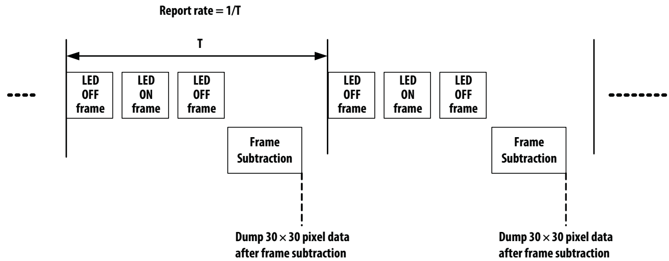
Figure 16. Timing of Output Image for 30 x 30 pixels.
