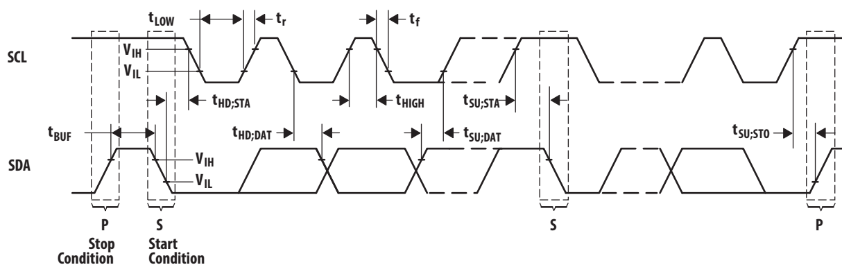
Figure 1. Timing Diagrams
