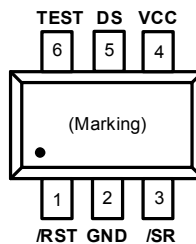
Top View SOT-26 / SC-70-6L
