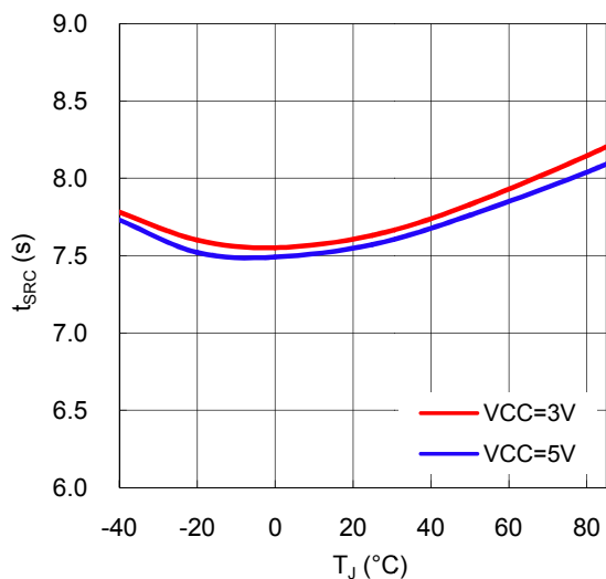
Fig.5 Reset Timer Delay vs. Junction Temperature
