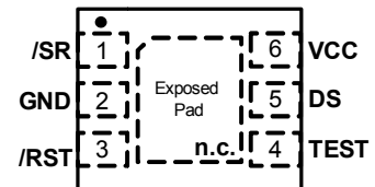
Top View DFN 1.5x2-6L
