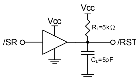
Fig.1 Test Circuit
