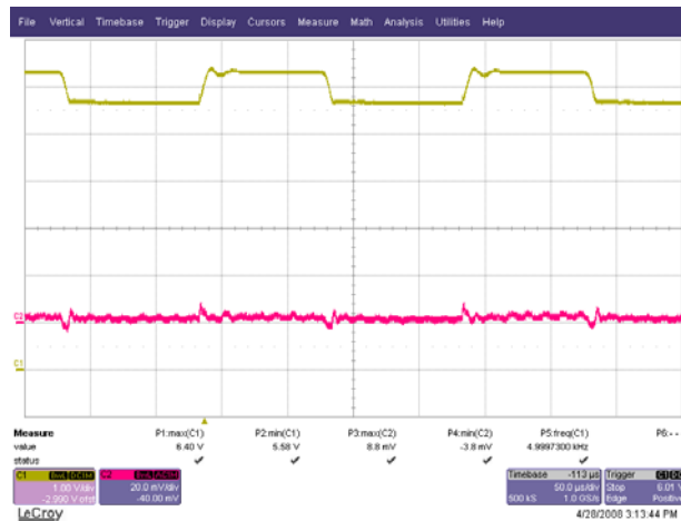
Line Transient
