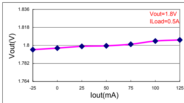
Load Regulation
