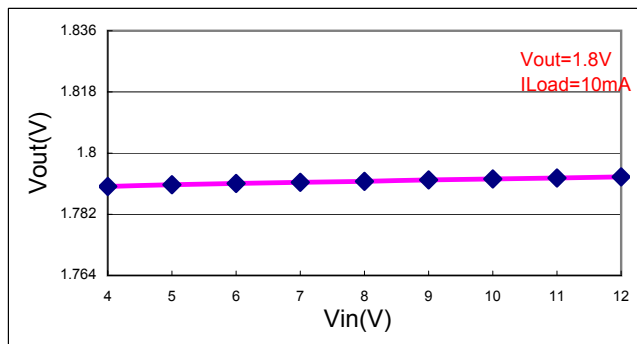
Line Regulation
