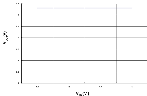
Line Regulation
