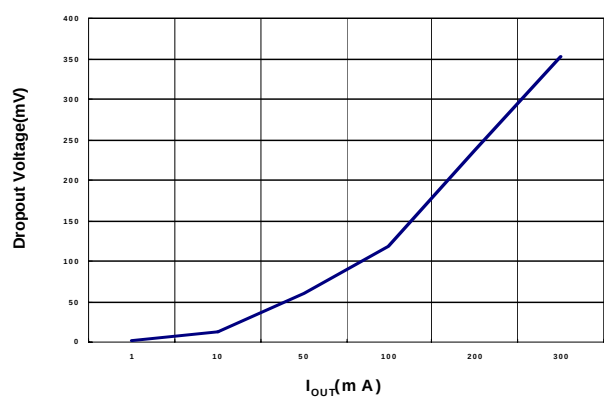
Dropout Voltage
