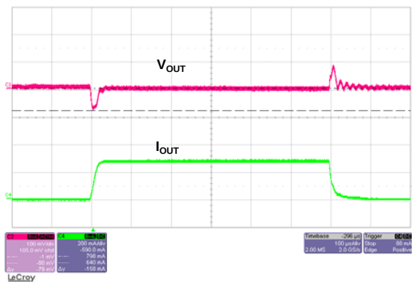
Load Transient
