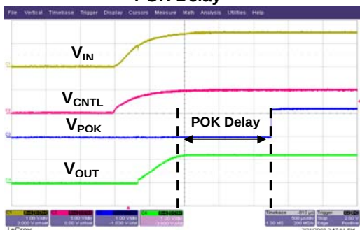
POK Delay
