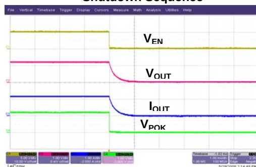
Shutdown Sequence
