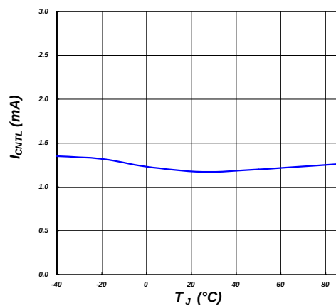
I_{CTL} vs. T_J
