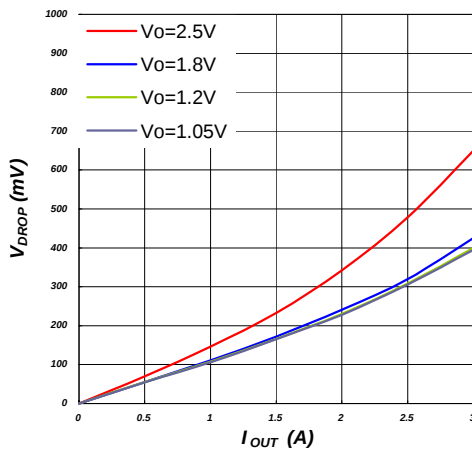
Dropout Voltage at V_{CTL} = 5\text{V}
