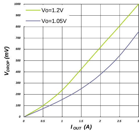
Dropout Voltage at V_{CTL} = 3.3\text{V}
