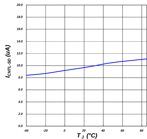
I_{CTL-SD} (APE8981MP-B) vs. T_J
