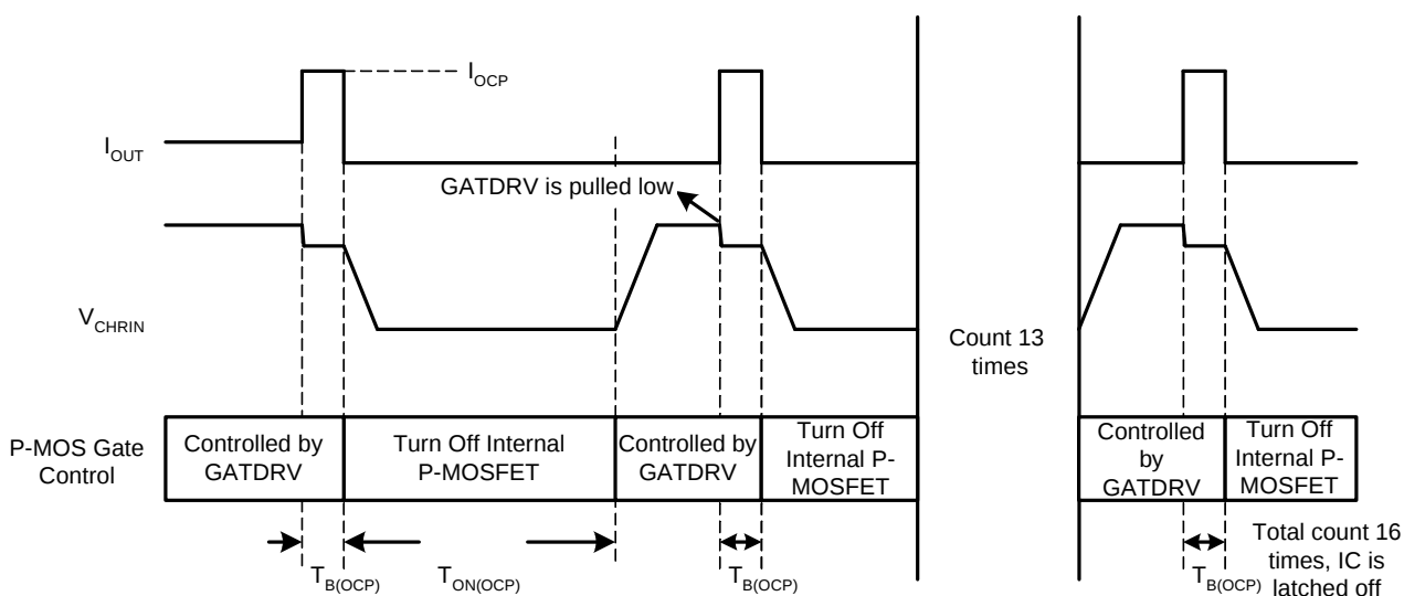
Figure 2. OCP Timing Diagram
