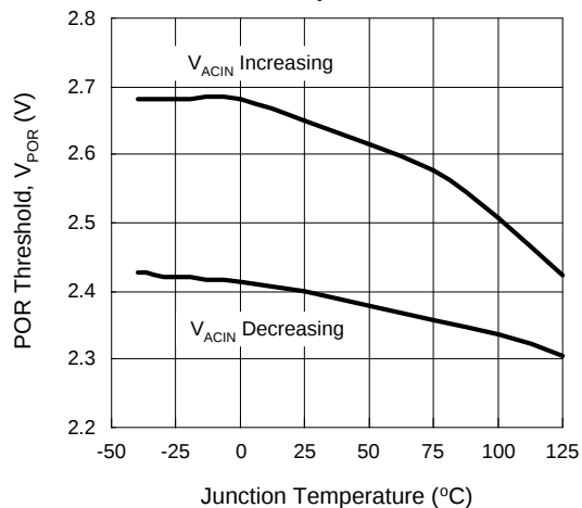
POR Threshold vs. Junction Temperature
