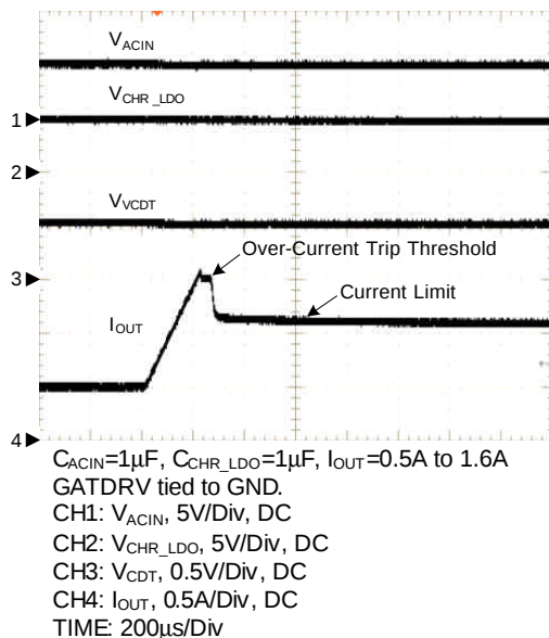
Current Limit Protection
