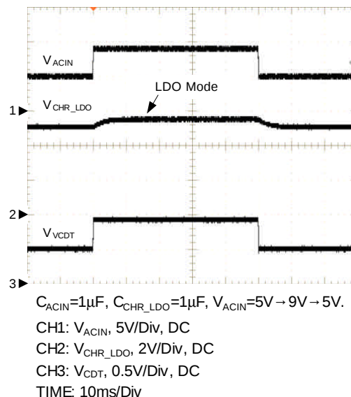
Input Line Transient Response
