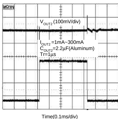
Load-Transient Response
