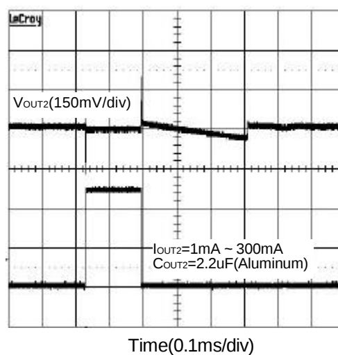
Load-Transient Response
