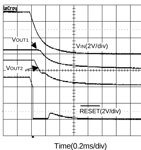
Powering Off
