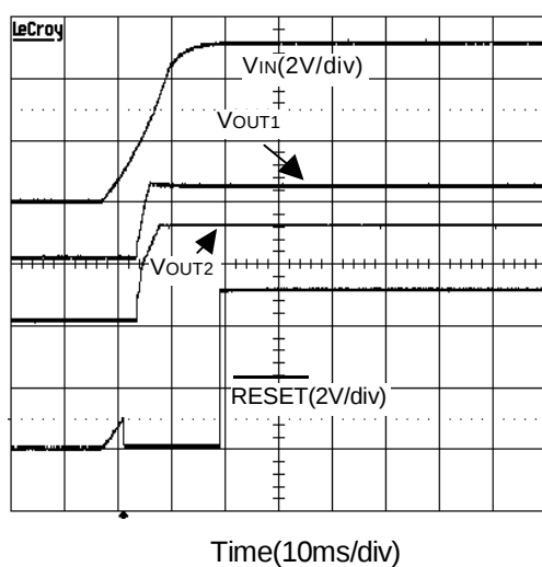
Powering On
