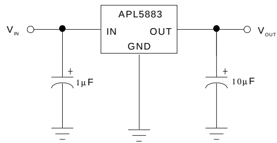
Fixed 2.85 and 3.3V Regulator
