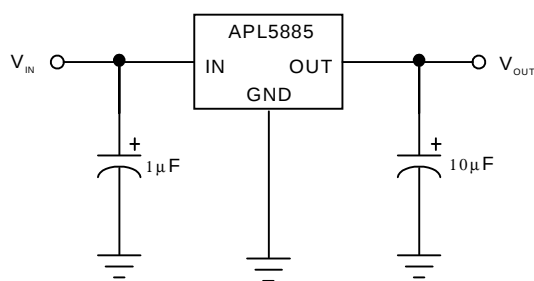
Fixed 1.8V, 2.5V and 3.3V Regulator
