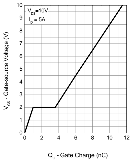
Gate Charge
