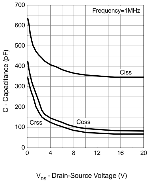
Capacitance
