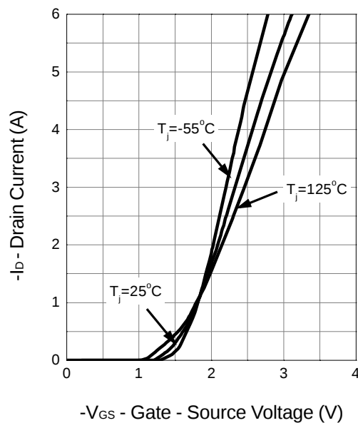
Transfer Characteristics
