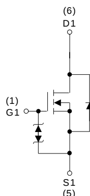
N-Channel MOSFET
