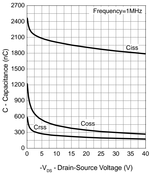
Capacitance
