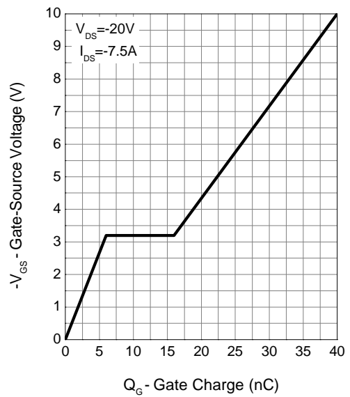
Gate Charge
