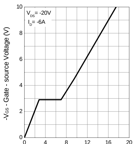
Gate Charge
