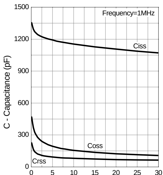
Capacitance
