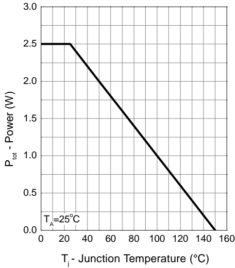
Power Dissipation
