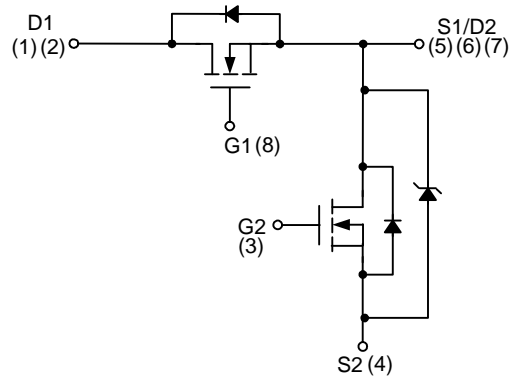
N-Channel MOSFET
