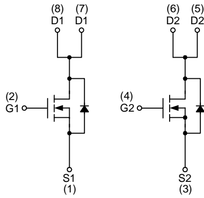
N-Channel MOSFET
