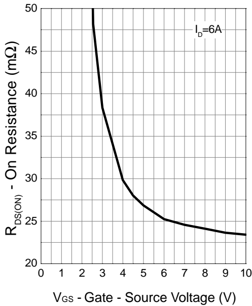
Transfer Characteristics
