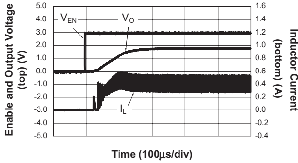
Soft Start
