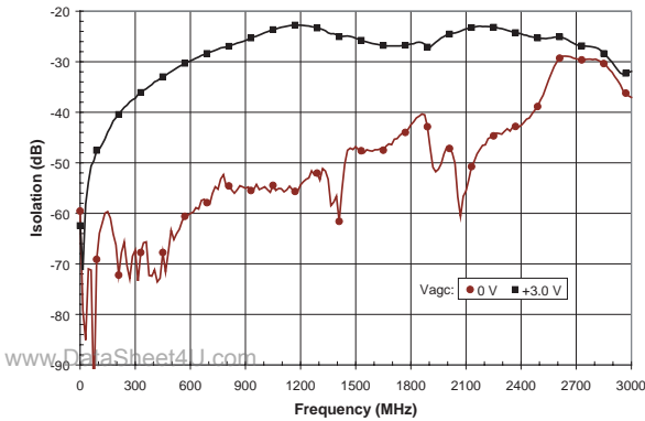
Figure 10: Output Port-to-Port Isolation vs. Frequency (T C = +25 °C, V CC = +5 V)
