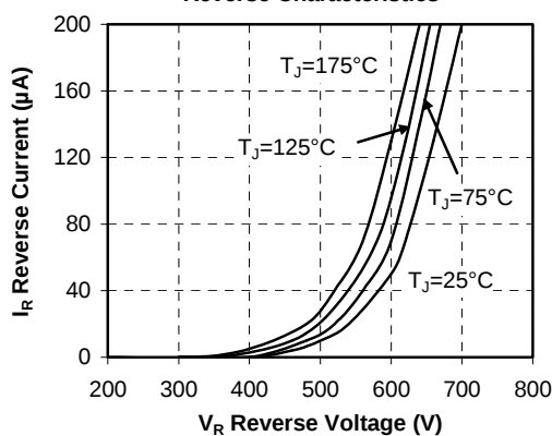
Reverse Characteristics
