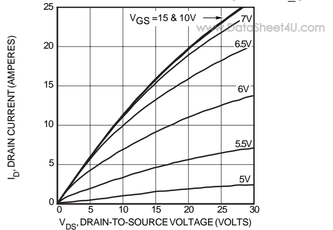
FIGURE 3, LOW VOLTAGE OUTPUT CHARACTERISTICS
