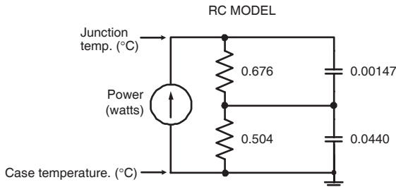
FIGURE 24b. TRANSIENT THERMAL IMPEDANCE MODEL
