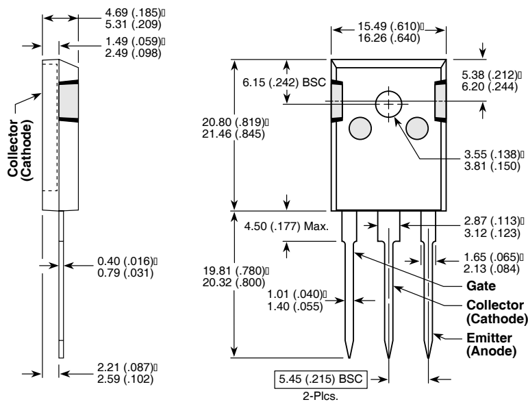
T0-247 Package Outline
