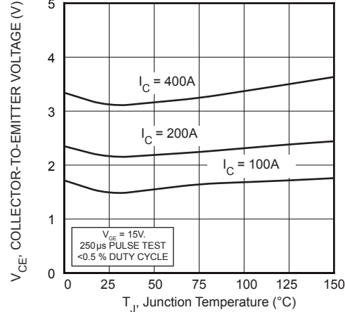
FIGURE 6, On State Voltage vs Junction Temperature
