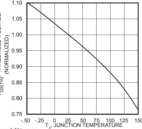
FIGURE 7, Threshold Voltage vs Junction Temperature
