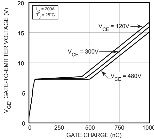
FIGURE 4, Gate charge
