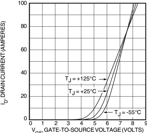
FIGURE 4, TRANSFER CHARACTERISTICS
