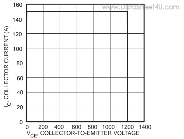
FIGURE 18, Minimum Switching Safe Operating Area
