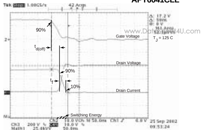
Figure 19, Turn-off Switching Waveforms and Definitions
