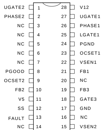
APW3007-12
