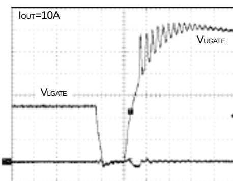
UGATE Rising
