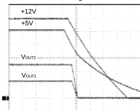
Powering OFF
