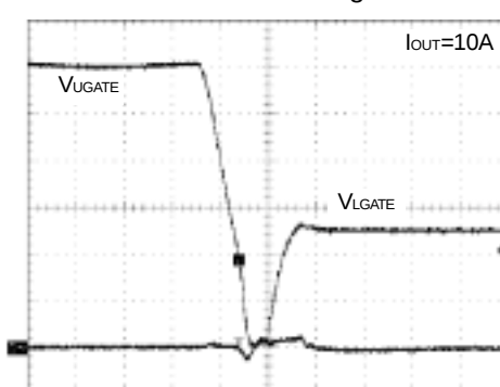
UGATE Falling
