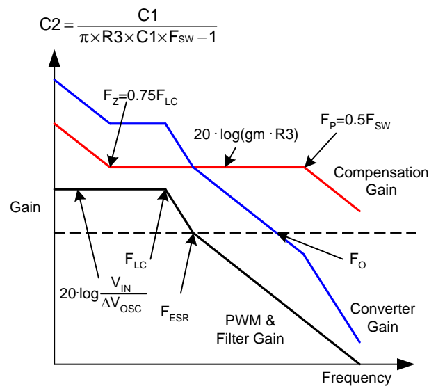
Figure 6. Converter Gain & Frequency
