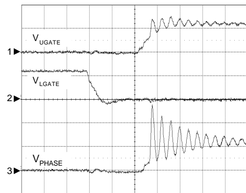
UGATE Rising
