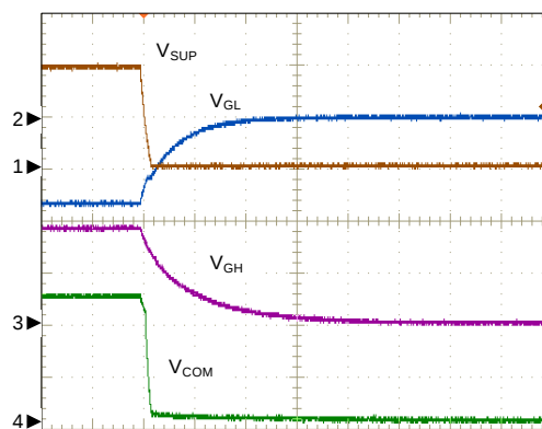
Power-Off Sequence
