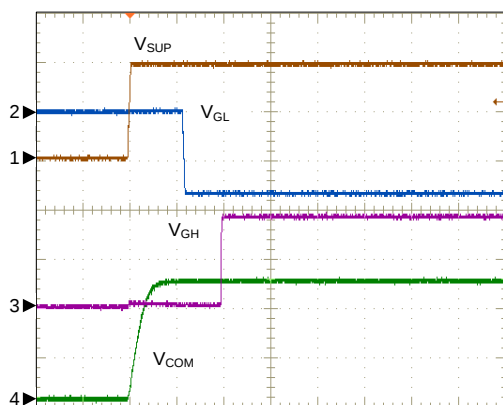
Power-On Sequence
