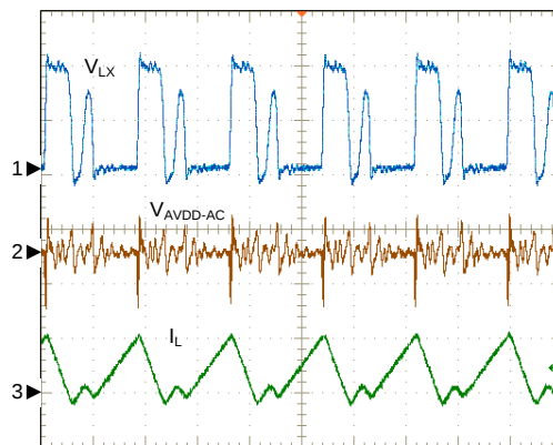
Boost Converter PWM Discontinuous Mode: Light Load
