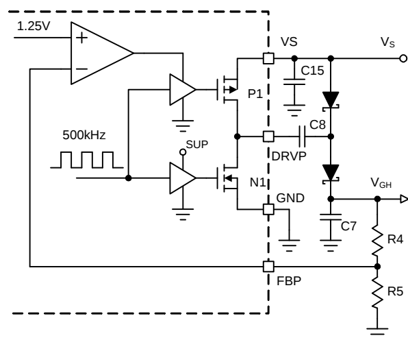
Fig1. Positive Charge Pump Regulator Block Diagram
