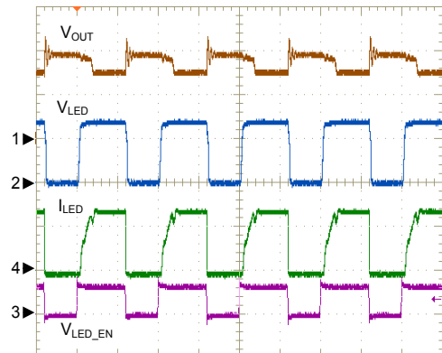
Dimming, 5KHz at 60% duty
