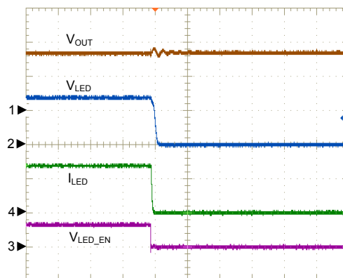
I LED Ramp-down at 0.5uS Slew Rate
