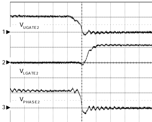
UGATEFalling
