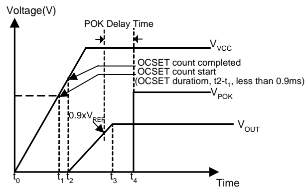
Figure 1. Soft-Start Interval
