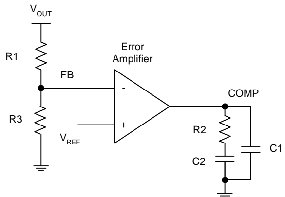
Figure 5. Compensation Network
