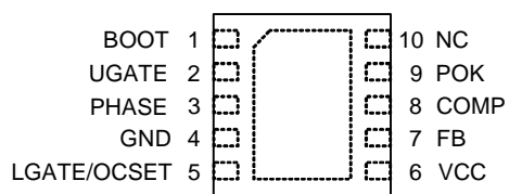
TDFN3x3-10 (Top View)
