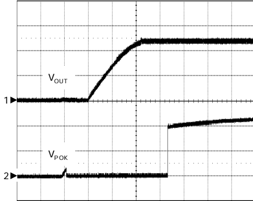
Power OK
