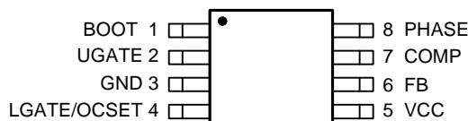
SOP-8 (Top View)
