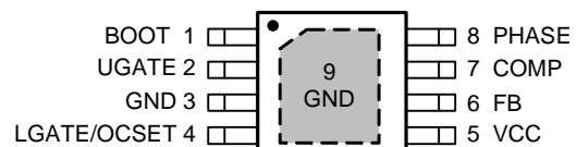
SOP-8P (Top View)
