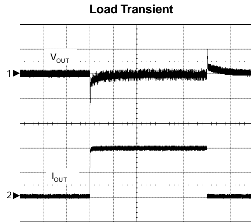
CH1: V_{OUT} , 50mV/Div, AC CH2: I_{OUT} , 5A/Div TIME: 200 \mu s/Div
