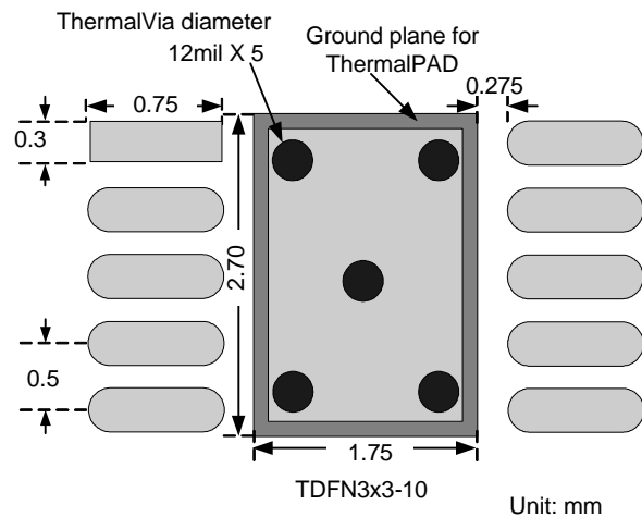
APW8805 Recommended Footprint
