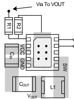
APW8805 Layout Consideration
