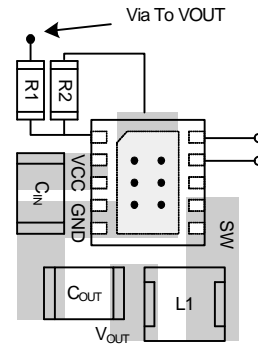
APW8805A Layout Consideration
